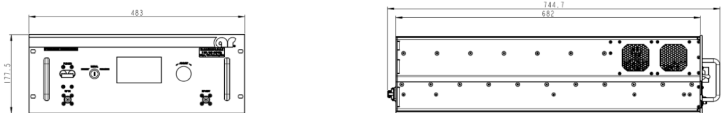
Units=mm; base model 4000SP1z2G1z4 shown
