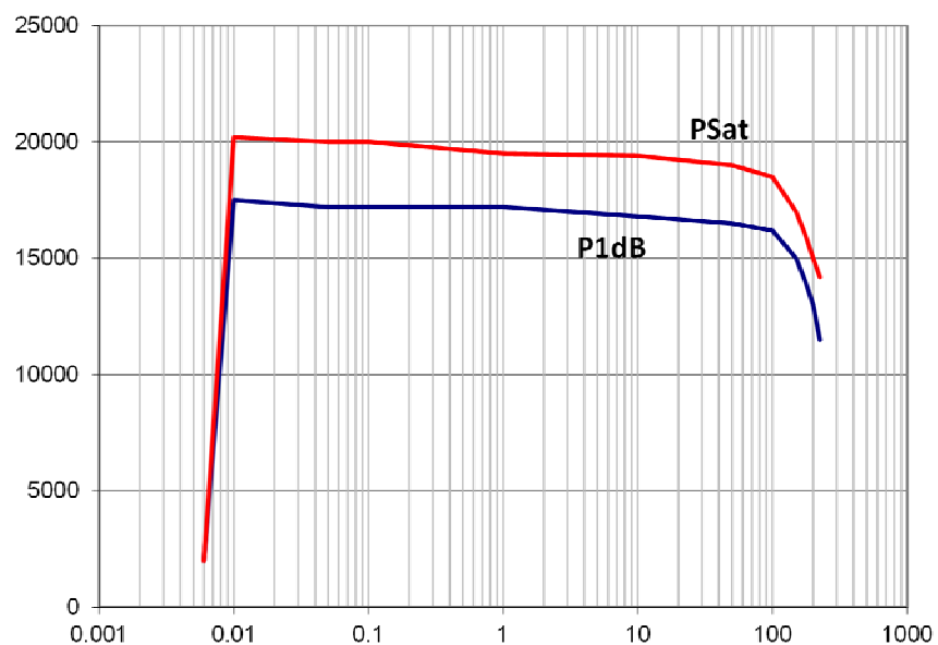
MODEL 20000A225A-L TYPICAL POWER OUTPUT
