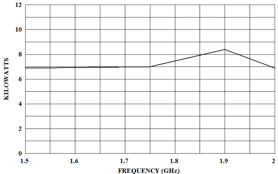
6500TP1z5G2 TYPICAL POWER OUTPUT
