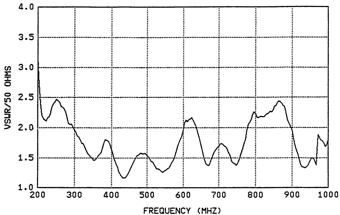
Model ATH200M1G-1 Antenna, Typical VSWR
