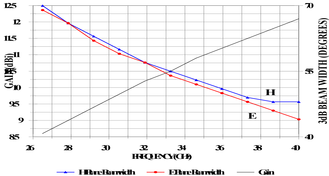
ATH26G40-1 GAIN & 3dB BEAMWIDTH VS FREQ
