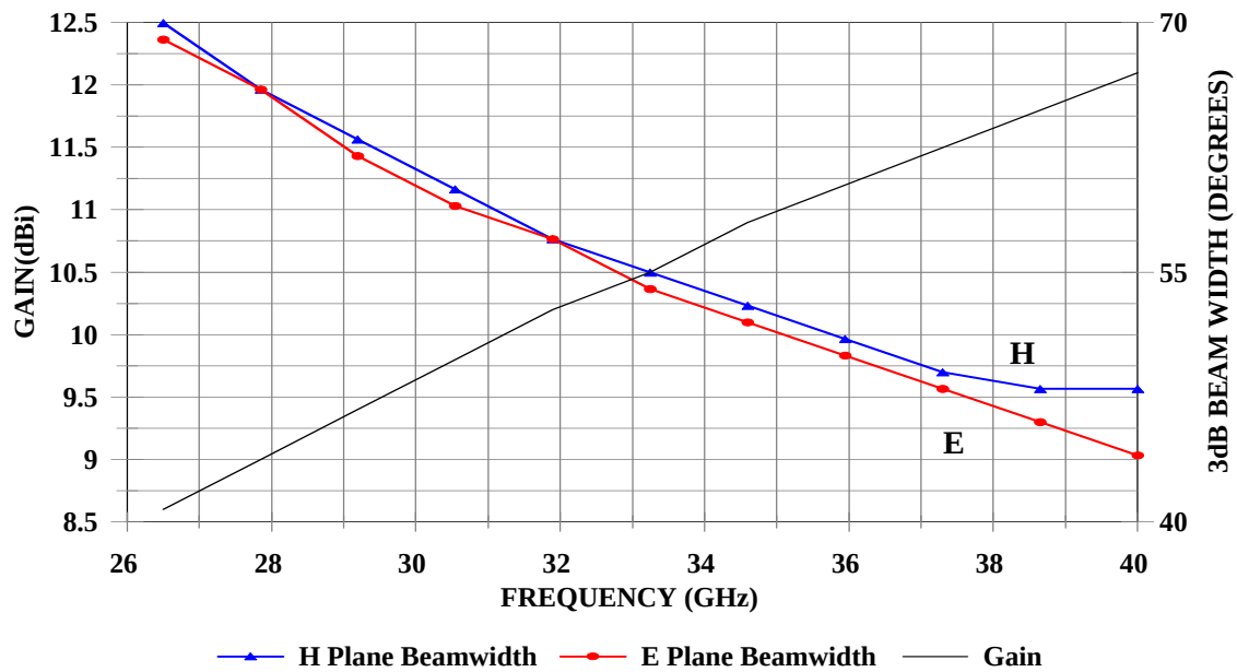
ATH26G40-1 GAIN & 3dB BEAMWIDTH VS FREQ
