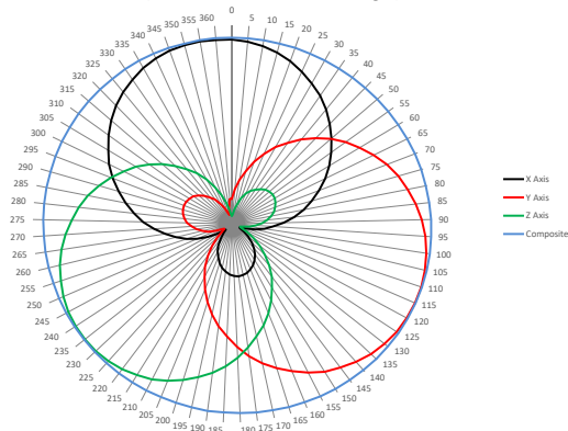
FL8060 Typical Isotropic Response at 100MHz (Rotated about the Ortho Angle)
