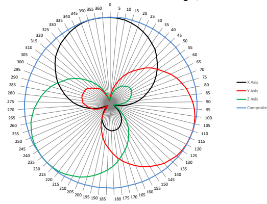
FL8200 Typical Isotropic Response at 10MHz (Rotated about the Ortho Angle)
