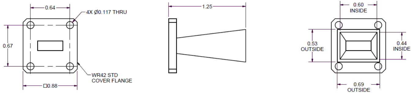
Drawing 10049830
