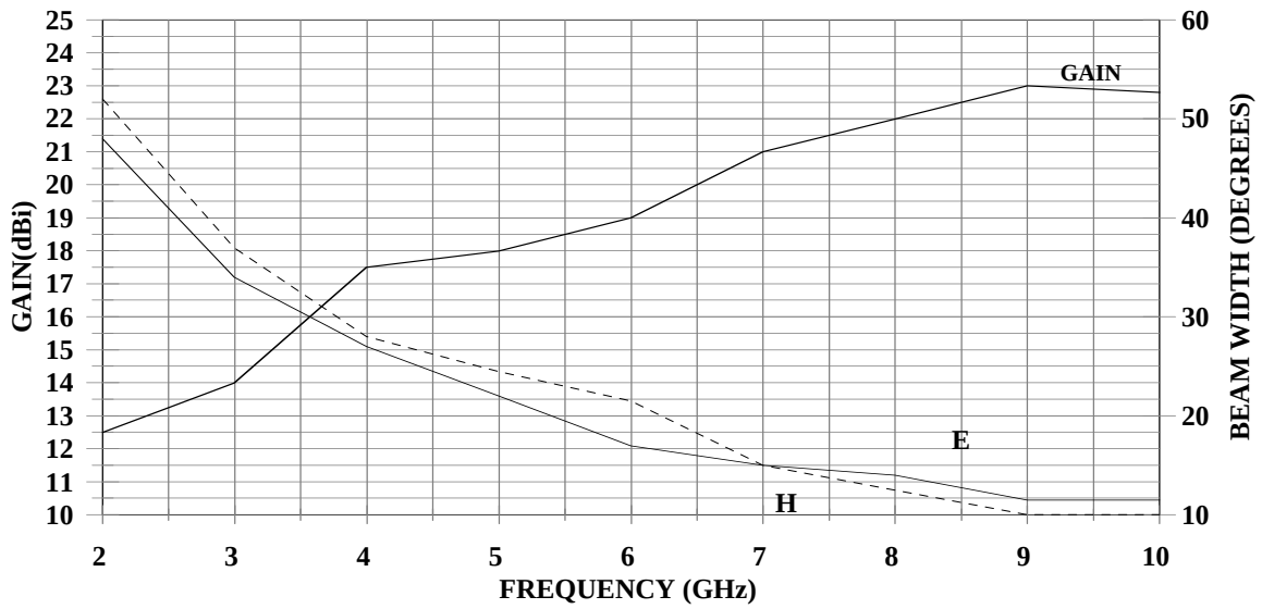
ATH2G10 GAIN & 3dB BEAM WIDTH VS FREQ
