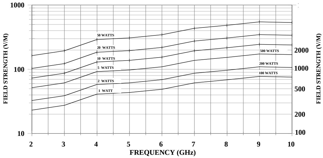
FIELD STRENGTH MEASURED AT 1 METER
