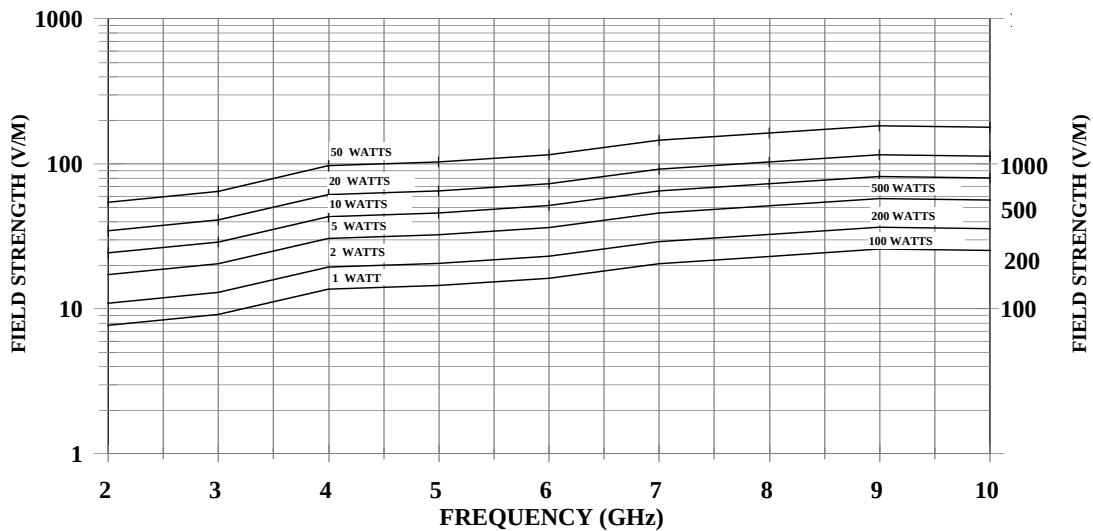
FIELD STRENGTH MEASURED AT 3 METERS
