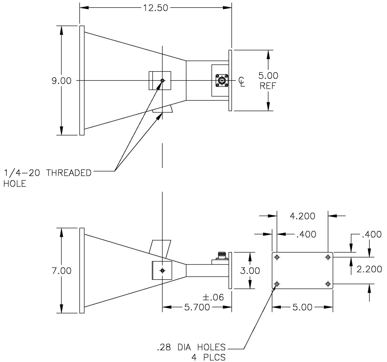
Outline Drawing 10013388, Rev A
