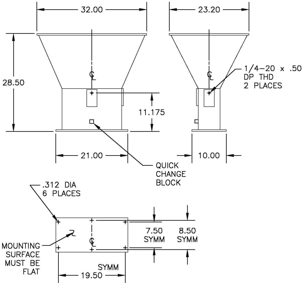
Drawing 10009155, Rev A
