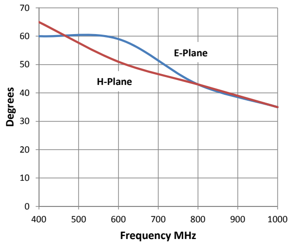
ATH400M1G 3dB Beamwidth
