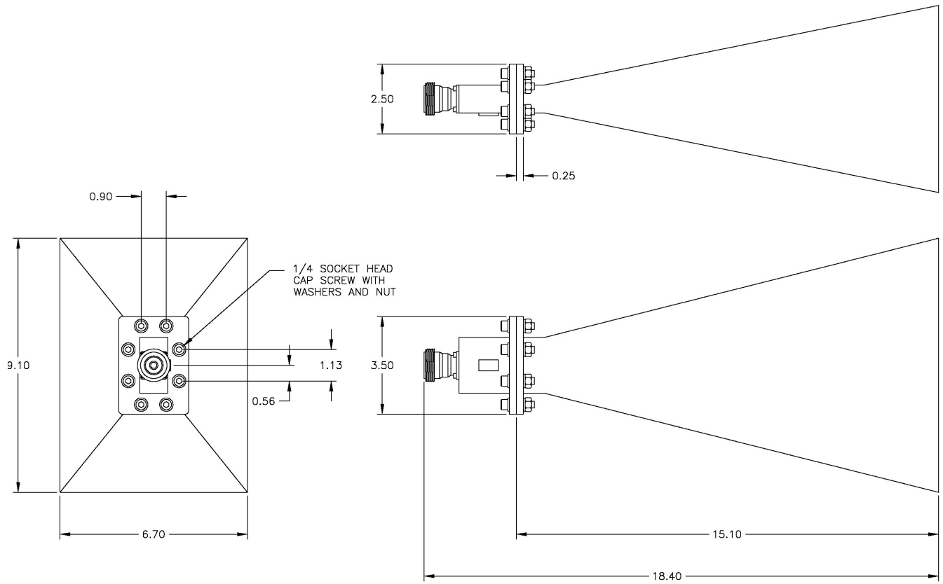
Drawing 10025819, Rev C
