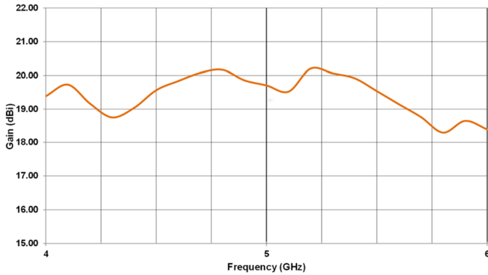
ATH4G6 Antenna Gain (dBi)
