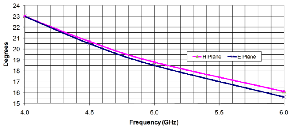
ATH4G6 3dB Beamwidth
