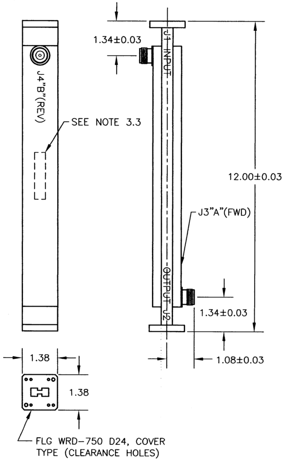
Model DC7450M1 Dimensions and Connector Locations
