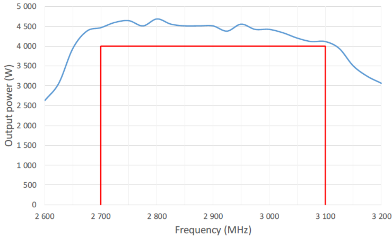
Typical Output Power (Psat @ 0 dBm input)
