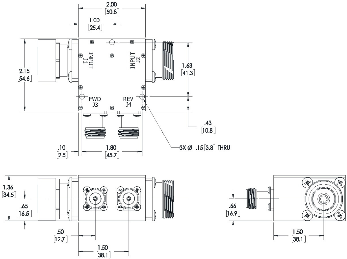
Drawing 10052792, Rev A
